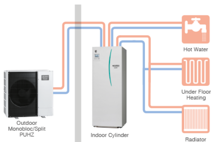
Figure 5. Air-Source Heat Pump Diagram
