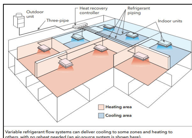
Figure 9. Typical VFR Schematic Diagram
